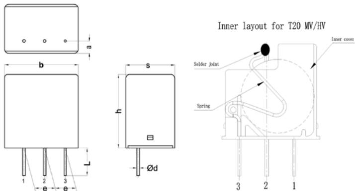
Outline drawing for T20 MV/HV*-types (see 1.2.1)
